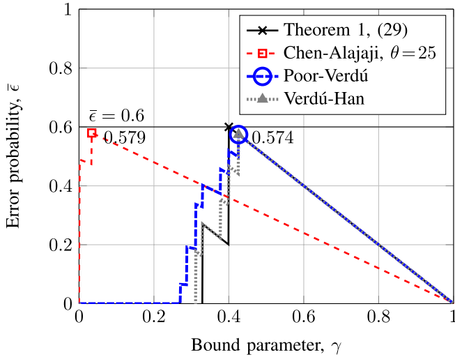
Fig. 1. Information-spectrum lower bounds to the minimum error probability for the example in Section III-A, as a function of the bound parameter \gamma .
