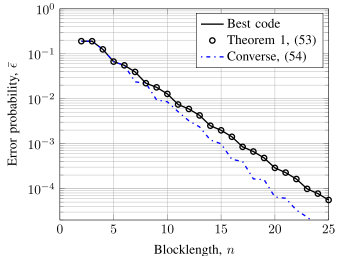
Fig. 2. Channel coding error probability bounds for a BSC with cross-over probability 0.1 and M = 4 codewords.
